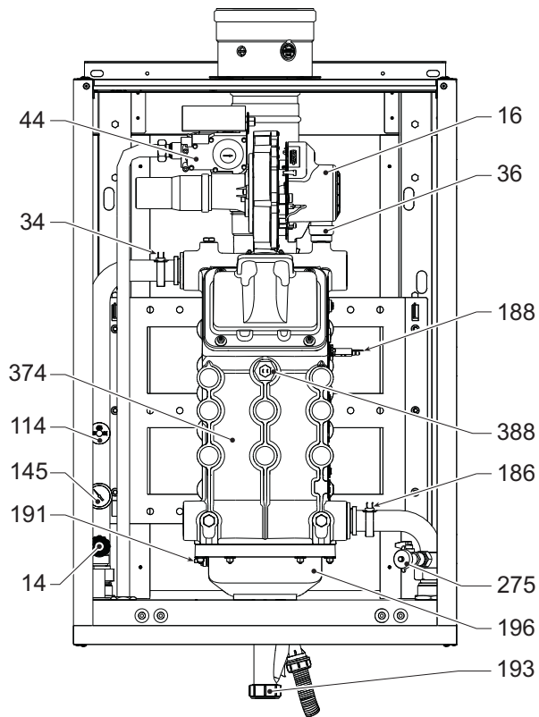
fig. 89- General view - model TORO W 60 and TORO W 80
