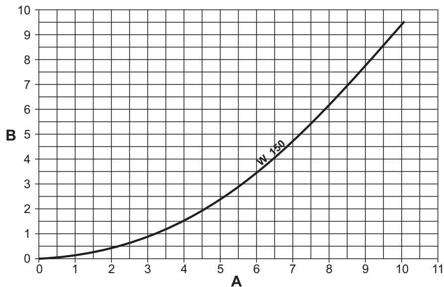
fig. 94- Pressure loss diagram - models TORO W 150
