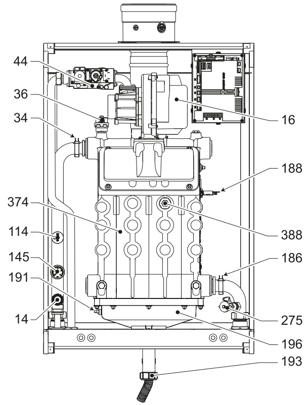
fig. 90- General view - model TORO W 99 and TORO W 120
