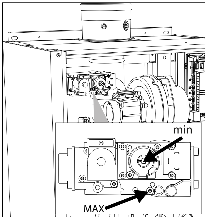
fig. 78- Maximum and minimum adjustment, models W 99, W 120 and W 150
