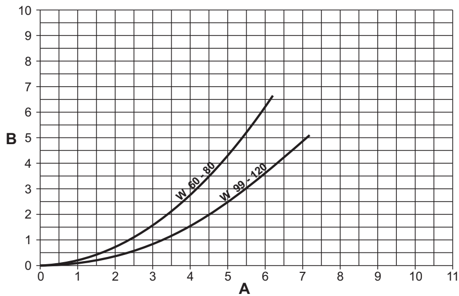
fig. 93- Pressure loss diagram - models TORO W 60 - TORO W 80 - TORO W 99 - TORO W 120
