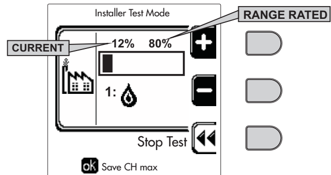
fig. 79- TEST mode (ex. heating power = 80%)
