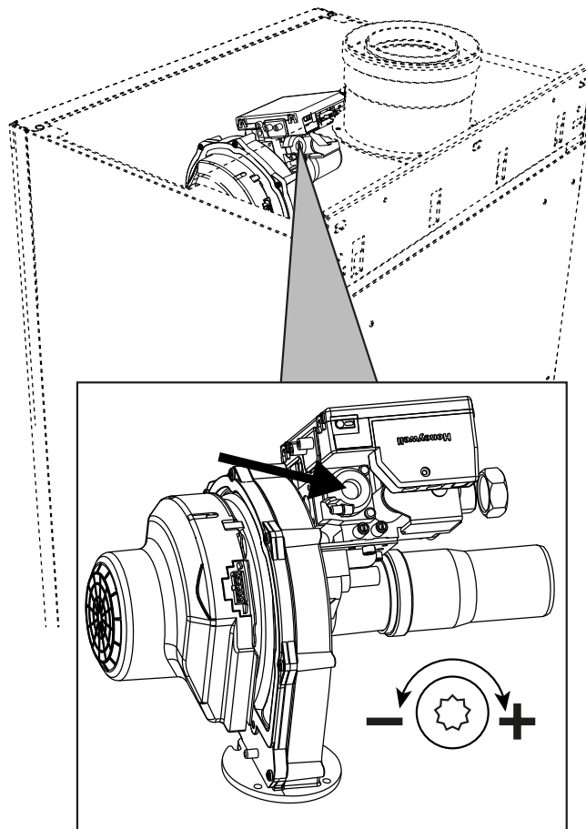
fig. 77- Minimum adjustment, models W 60 and W 80
