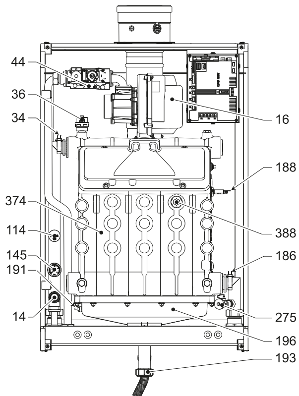
fig. 91- General view - model TORO W 150
