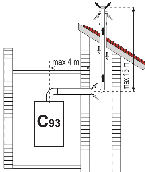
fig. 62- Examples of connection to collective flues (⇐ = Air / ⇨ = Fumes)
