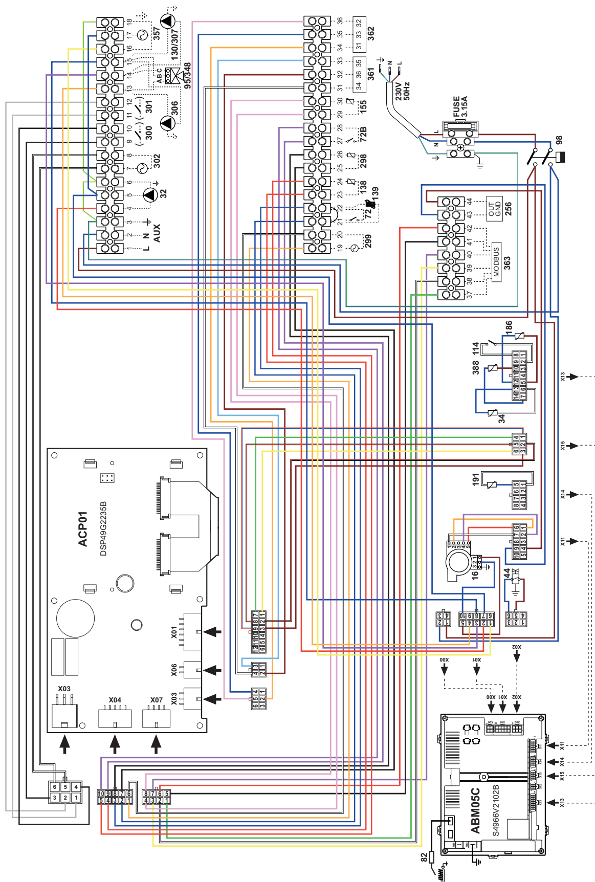
fig. 100- Wiring diagram - models TORO W 99, TORO W 120 and TORO W 150
